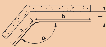
Single bend
